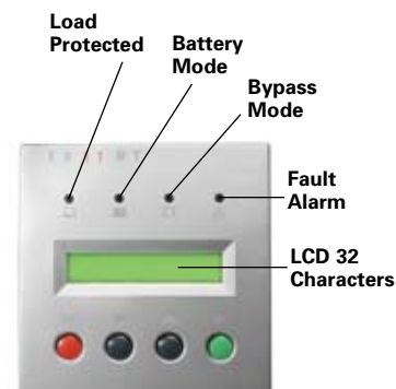
Front panel LCD control panel LCD, rotating (tower/rack format), multilingual, backlit
