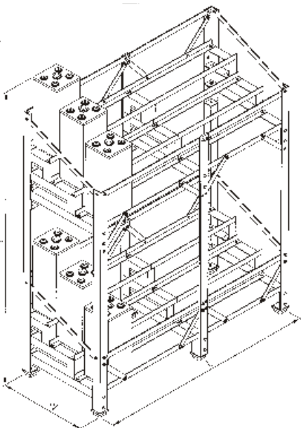
3 step, 2 tier rack
