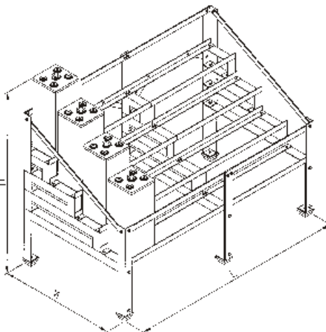
4 step, 1 tier rack
