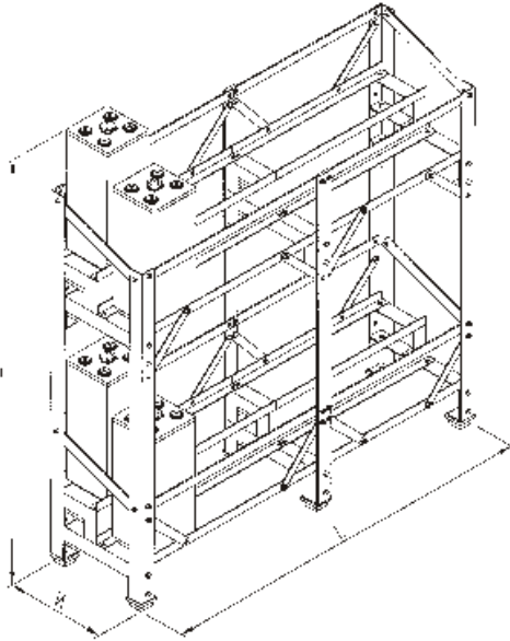
2 step, 2 tier rack
